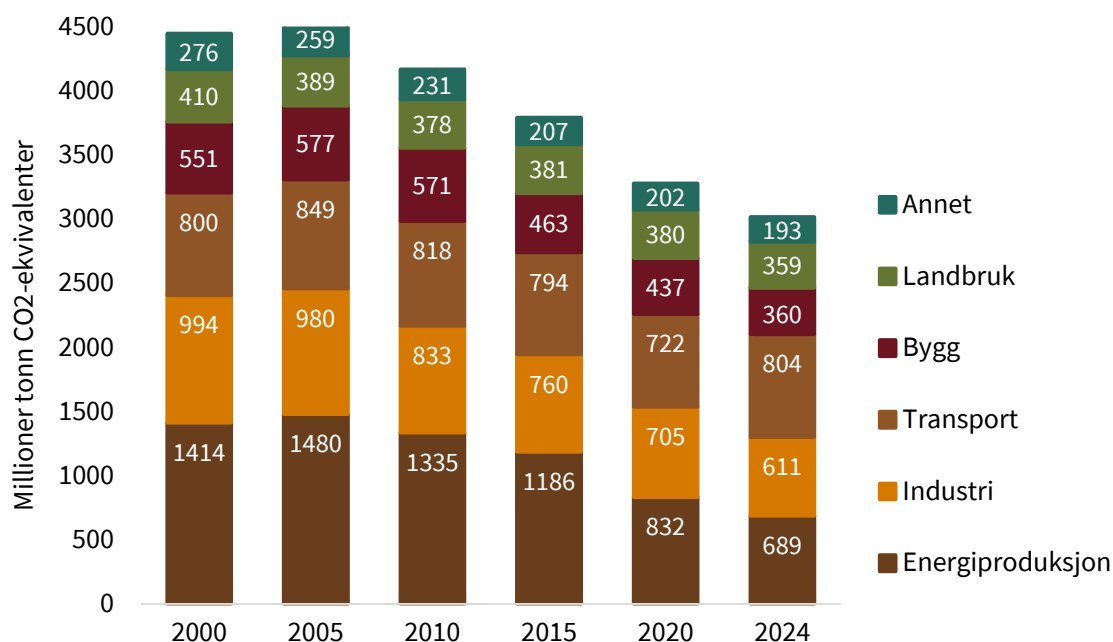
Figur 4-3 Klimagassutslipp i EU27. Kilde: European Environment Agency.
