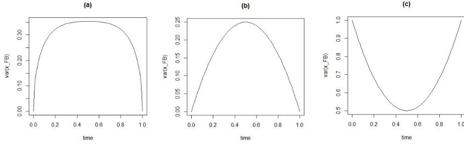
Figure 2: Prediction variance as a function of time. Here, time is scaled so that t=0 is the start of the gap, t=1 is the end of the gap. Figure 2a shows the interpolation variance when the forward and backward prediction variance respectively are v_F(t) \propto \sqrt{t} and v_B(t) \propto \sqrt{1-t} . Figure 2b shows the interpolation variance when the forward and backward prediction variance respectively are vv_{FF}(tt) \propto tt and vv_{BB}(tt) \propto 1-tt . Figure 2c shows the interpolation variance when the forward and backward prediction variance both are constant, so vv_{FF}(tt) = vv_{BB}(tt) = cc .
