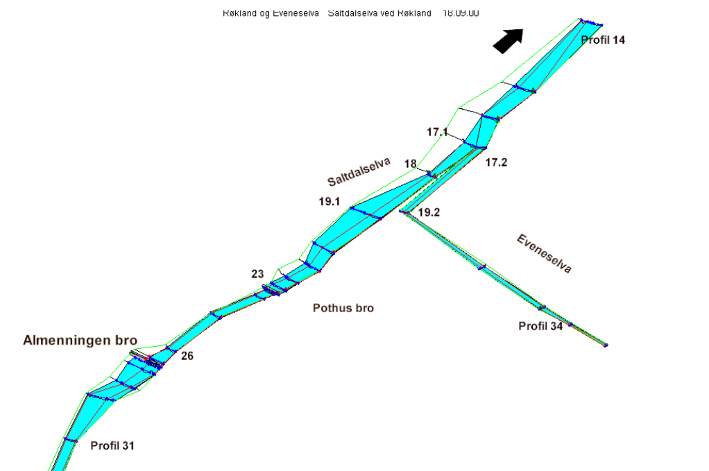
Figur 3-9, HEC-modell for Røkland.
